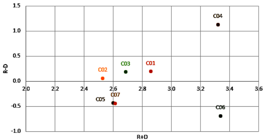
Fig 2: The causal diagram from the crisp data for main Criteria
