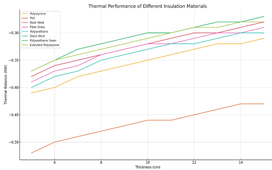
Diagram 1: Wall types simulation results (source: authors)
