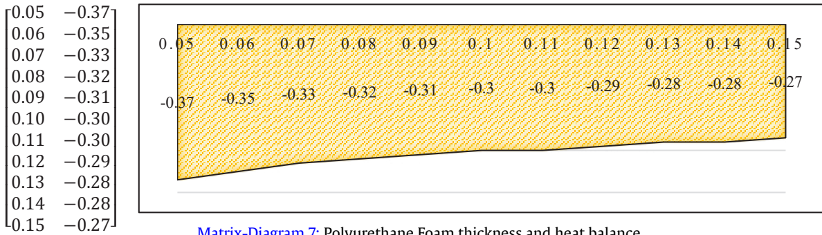
Matrix-Diagram 7: Polyurethane Foam thickness and heat balance
