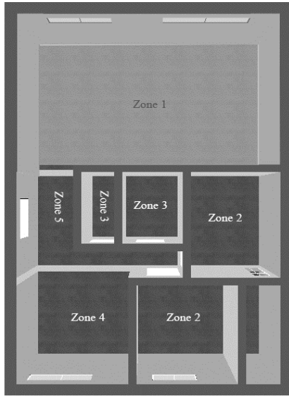
Fig. 2: building plan 2d model zoning (source: author)
