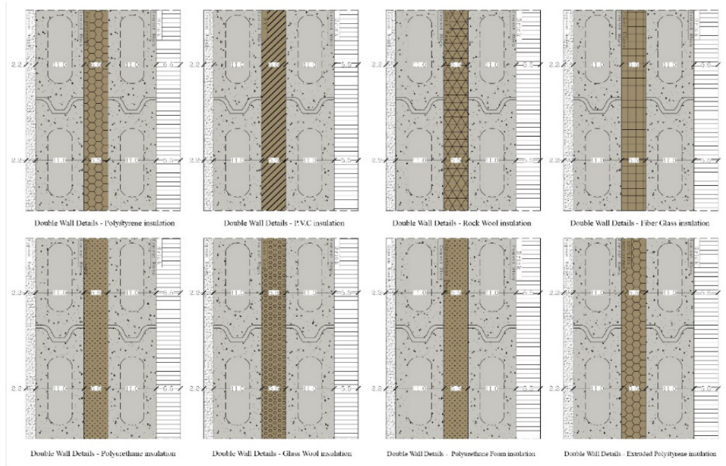
Fig. 3: Eight wall types with different insulation materials (source: authors)
